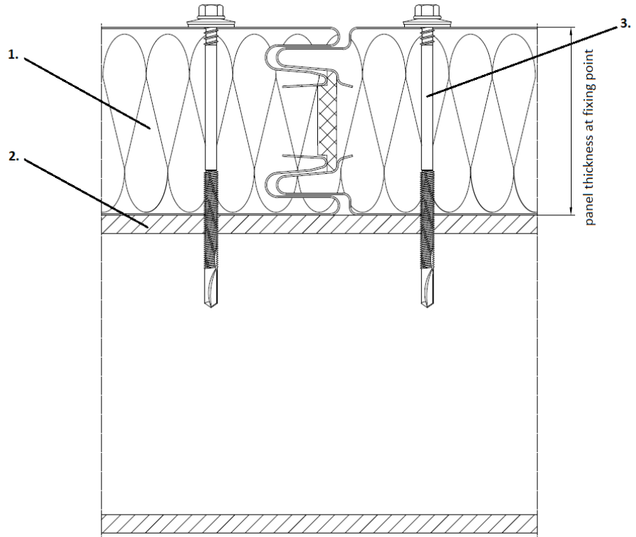
Picture 1. Assembling of the M12S-SP with wall sandwich panel on steel substrate with use of MSD stress diffuser.
