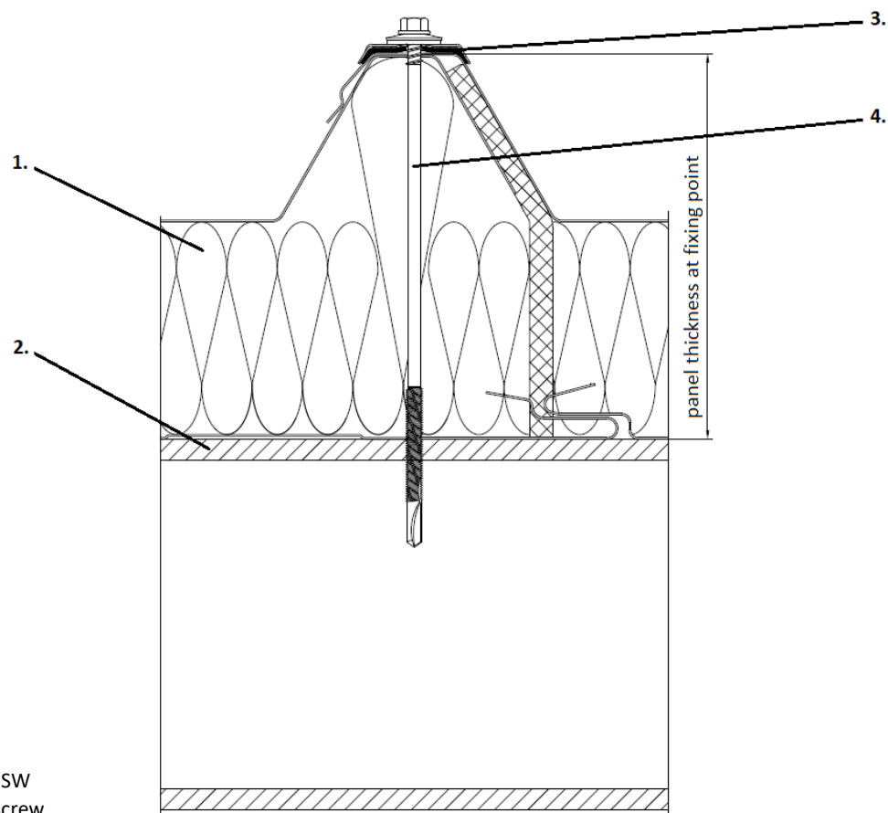
Picture 3. Assembling of the M12S-SP with roofing sandwich panel on steel substrate with use of MSW saddle washer - cross section across the sandwich panel.
